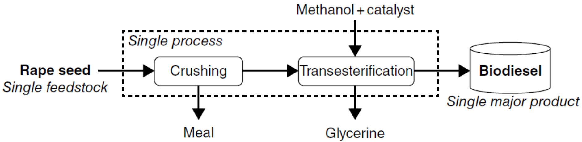
The biodiesel process: an example of a phase I biorefinery.
