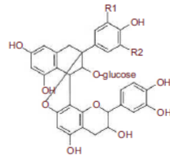
Anthocyanin-flavanol adduct (A-T)
