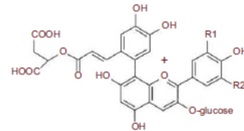
Caftaric acid-anthocyanin adduct
