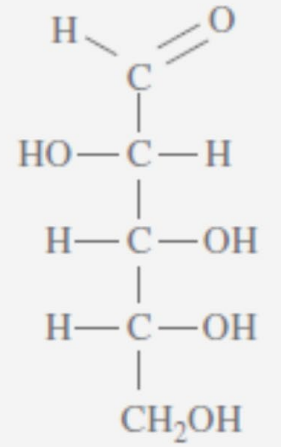
Arabinose
