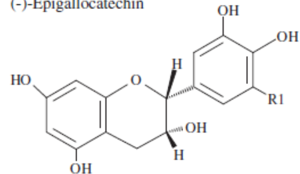
(-)-Epicatechin (2R, 3R) (-)-Epigallocatechin
