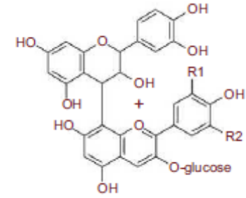
Flavanol-anthocyanin adduct (T-A)
