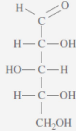
Xylose
