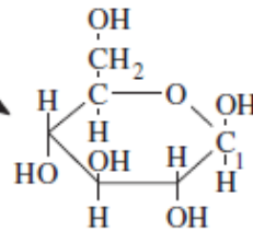
\beta -Glucopyranose D-Glucose (Haworth projection)
