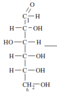
D-Glucose (Fischer projection)
