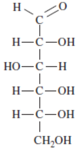
Glucose
