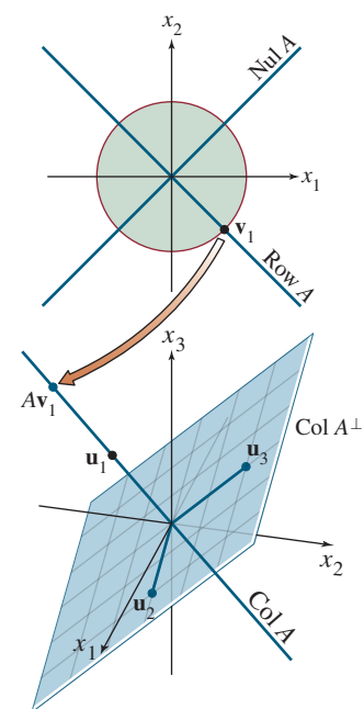
The fundamental subspaces in Example 4.
