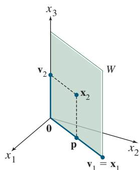
FIGURE 1 Construction of an orthogonal basis \{v_1, v_2\} .
