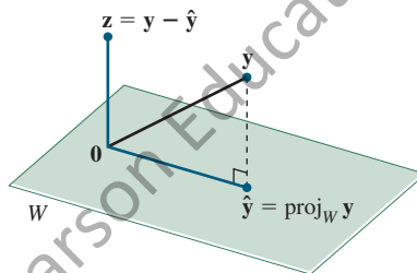
FIGURE 2 The orthogonal projection of \mathbf{y} onto W .
