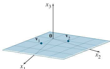
FIGURE 10 An example of a subspace.
