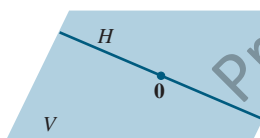
FIGURE 6 A subspace of V .
