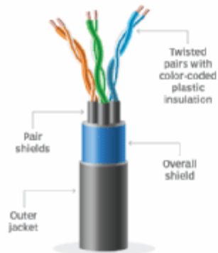
Shielded twisted pair
