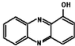
Micyanine
