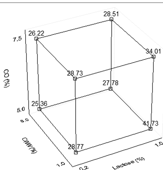
Fig. 2 Cubic plot of the surface tension values estimated from the full-factorial design of Table 2
