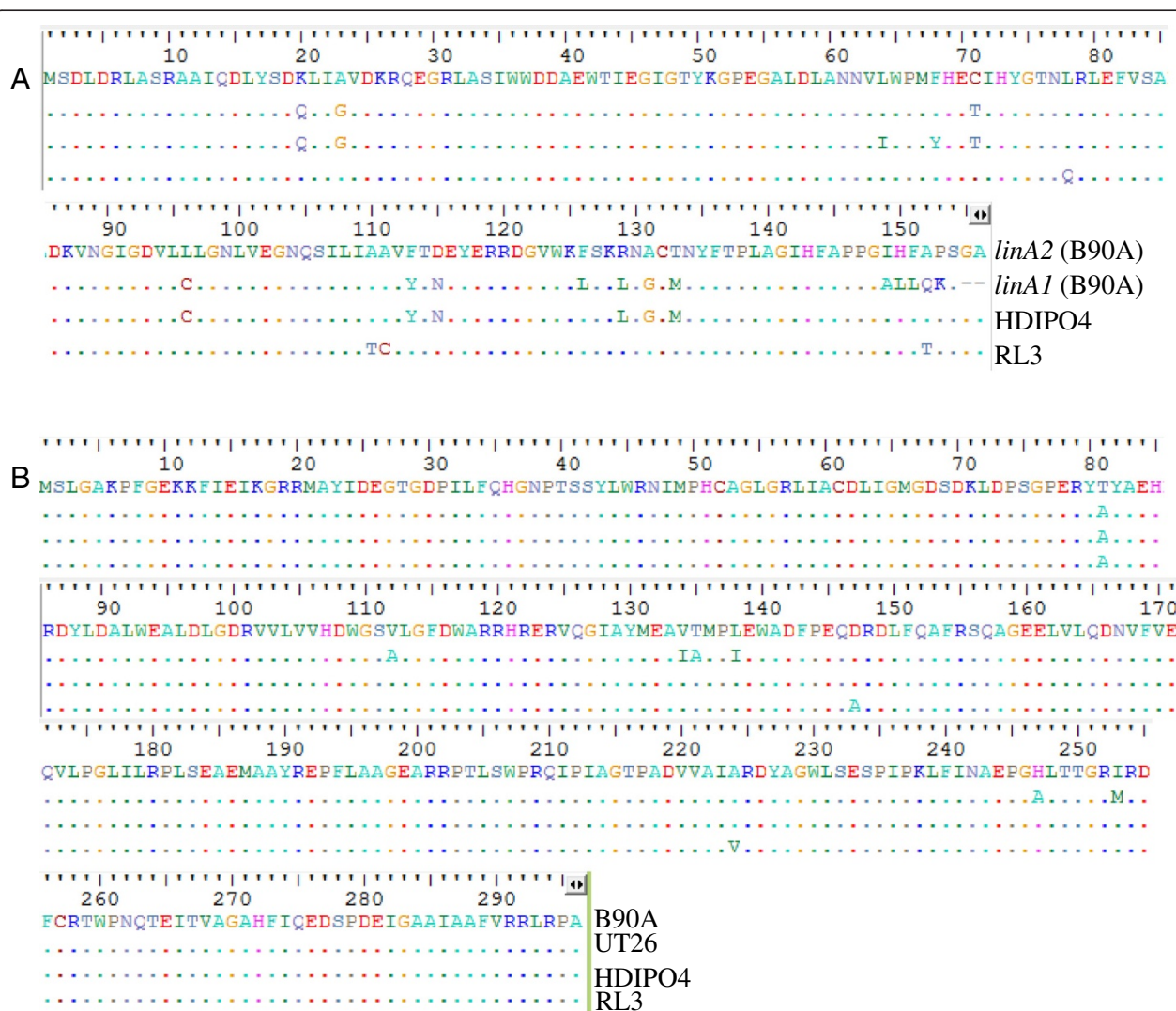
Figure 7 A) Multiple sequence alignments of linA B) linB gene sequences in the strains showing variation. Amino acid sequences of linA and linB genes from the strains were aligned using BioEdit to depict the substitutions at the respective sites.
