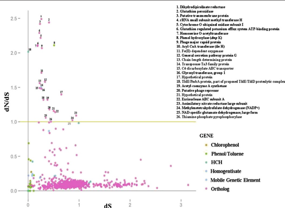
Figure 10 dN/dS v/s dS plot of orthologs, xenobiotic degradation pathway genes and IS elements/integrases. Sequences of orthologs, xenobiotic degradation pathway genes and IS elements/Integrases were used for calculating their dN/dS. Genes having dN/dS value >1 are under positive natural selection.
