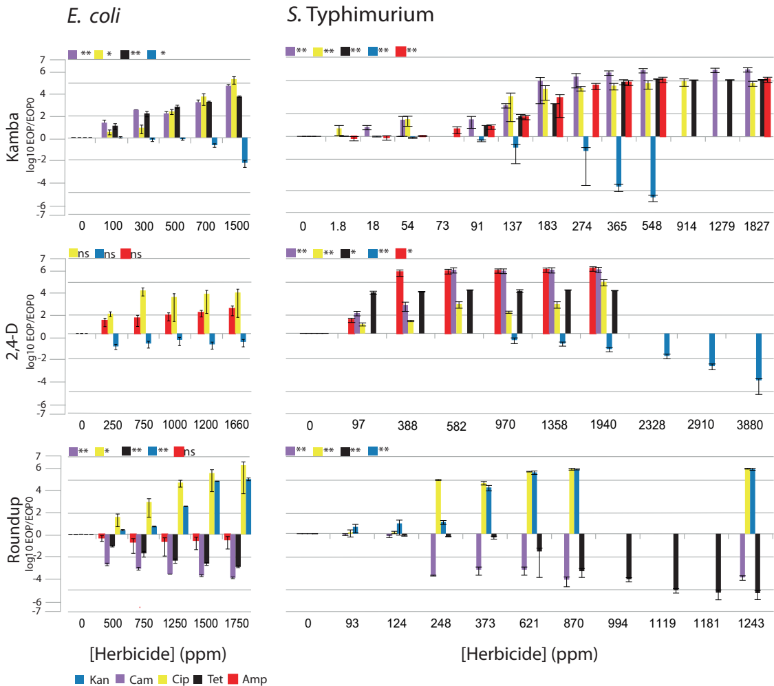
FIG 2 Dose-response curves. Antibiotic concentrations used (in μg/ml) were as follows: with 2,4-D, Amp at 4/40 ( S. Typhimurium / E. coli ), Cip at 0.003/0.003, Cam at 4.4/-, Kan at 6/2.5, and Tet at 0.75/-; with Kamba, Amp at 2/0, Cip at 0.03/0.05, Cam at 4/20, Kan at 2/1, and Tet at 0.75/3; and with Roundup, Amp at -/20, Cip at 0.05/0.07, Cam at 2/10, Kan at 12/10, and Tet at 0.45/1. Error bars are SEM, and asterisks indicate P values (see Materials and Methods for details). *, P < 0.05 ; **, P < 0.01 ; ***, P < 0.001 ; ns, not significant; -, not tested.
