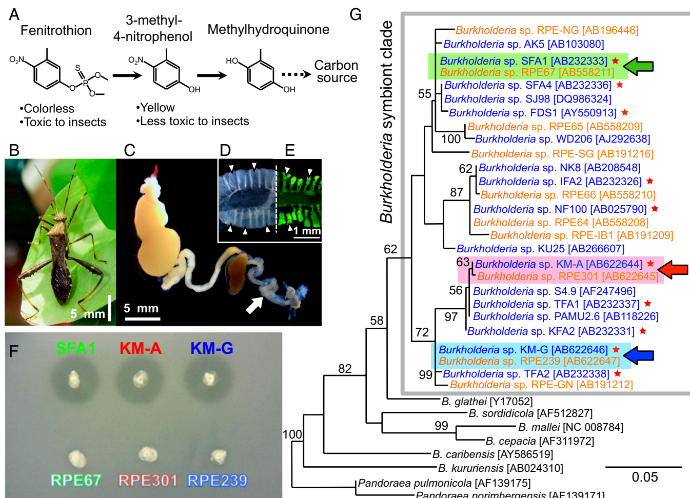
Fig. 1. Fenitrothion degradation by Burkholderia , and Burkholderia gut symbiont of R. pedestris . (A) Fenitrothion degradation pathway in soil-derived Burkholderia (10, 18). (B) An adult male of R. pedestris . (C) A dissected alimentary tract of R. pedestris . An arrow indicates midgut fourth section as symbiotic organ. (D) An enlarged image of the symbiotic organ. (E) Localization of Burkholderia in the midgut crypts. Arrowheads indicate midgut crypts in D and E. (F) Halo formation by fenitrothion-degrading Burkholderia strains on a fenitrothion-containing agar plate. (G) Phylogenetic relationship of symbiotic Burkholderia strains from R. pedestris (orange) and soil-derived Burkholderia isolates (blue). Stars indicate fenitrothion-degrading strains. A maximum likelihood phylogeny inferred from 1,228 aligned nucleotide sites of 16S rRNA gene sequences is shown with bootstrap values. Closely related pairs of fenitrothion-degrading and nondegrading Burkholderia strains used in this study are highlighted by colored arrows: SFA1 and RPE67 in green, KM-A and RPE301 in red, and KM-G and RPE239 in blue.
