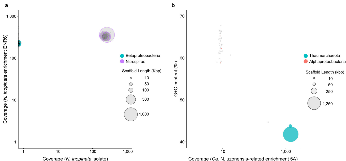
Extended Data Figure 1 | Binning of the metagenome scaffolds from nitrifier cultures. Circles represent scaffolds, scaled by the square root of their length. Only scaffolds \geq 5 kbp are shown. Clusters of similarly coloured circles represent potential genome bins. a , Sequence-composition-independent binning of the scaffolds from the N. inopinata isolate. The previous enrichment culture ENR6, which contained N. inopinata and only one contaminating betaproteobacterial organism 1 , was used for comparison in differential coverage binning. The lack of scaffolds from the betaproteobacterium (coverage = 0) shows the absence of this organism in the pure culture of N. inopinata . To further confirm that no trace amounts of the betaproteobacterium were left in the pure culture, the trimmed sequence reads were also mapped to the ENR6 metagenomic assembly that contained the contaminant 1 . None of
