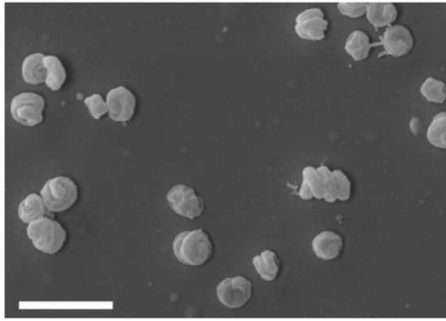
Extended Data Figure 2 | Morphology and completely nitrifying activity of the N. inopinata isolate. a , Scanning electron micrograph of spiral-shaped N. inopinata cells. The cells had a diameter of 0.2 to 0.3 \mu\text{m} and length of 0.7 to 1.7 \mu\text{m} . The scale bar represents 2 \mu\text{m} . b , Near-stoichiometric
