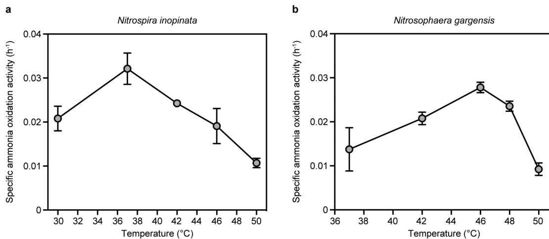
Extended Data Figure 3 | Temperature optima of the ammonia-oxidizing activity of N. inopinata and N. gargensis . a , Ammonia oxidation by N. inopinata over a temperature range from 30 to 50 ^{\circ}\text{C} . Since the optimum for activity was at 37 ^{\circ}\text{C} , kinetic analyses of N. inopinata were performed at this temperature. b , Ammonia oxidation by N. gargensis
