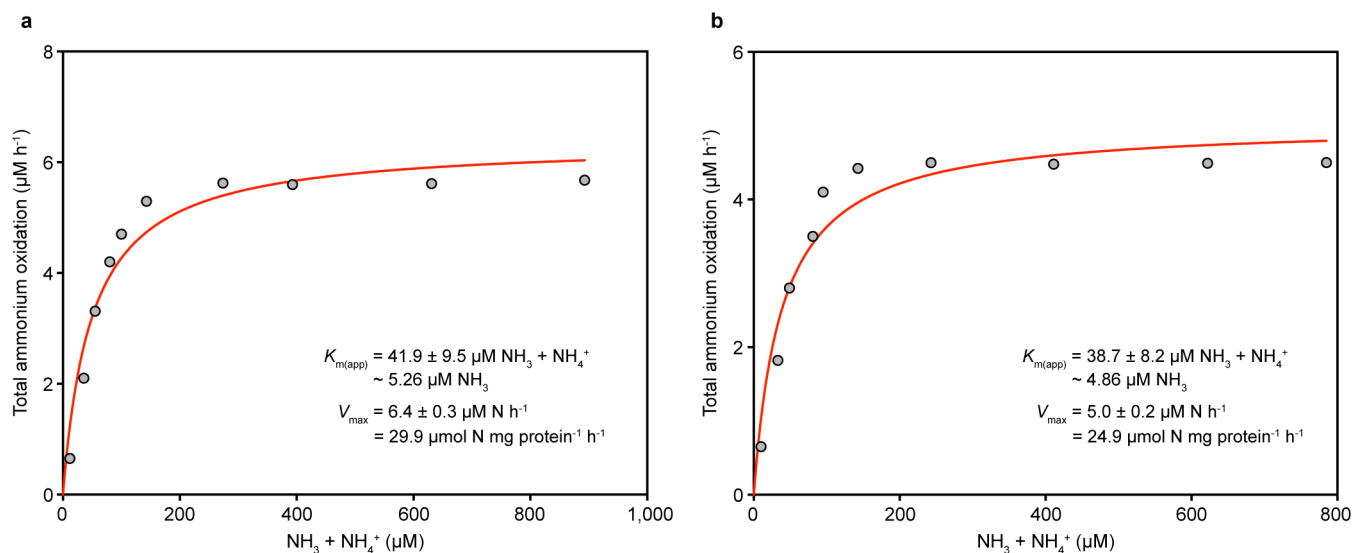
Extended Data Figure 8 | Ammonia oxidation kinetics of ‘ Ca. Nitrosotenuis uzonensis ’. Apparent half-saturation constants ( K_{m(\text{app})} ) and maximum oxidation rates ( V_{\text{max}} ) for total ammonium were determined by fitting the data to the Michaelis–Menten kinetic equation. The red curve indicates the best fit of the data. Standard errors of the estimates based on nonlinear regression are reported. See Methods for details of experiments and calculations. a , b , Total ammonium oxidation
