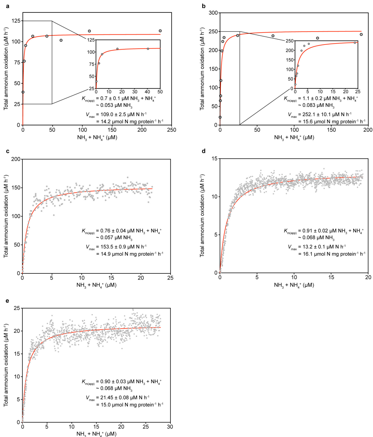
Extended Data Figure 4 | Ammonia oxidation kinetics of N. inopinata .
