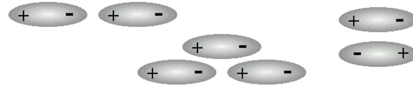
Attractive Dipole-Dipole Interactions
