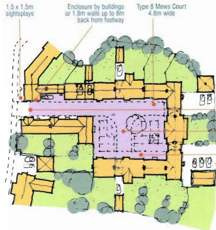
Mews court more than 20m long
