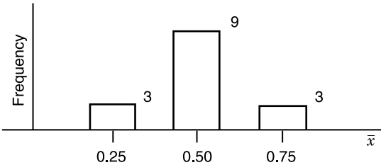
Figure 4.2 Normal shape of sampling distribution for Example 4.1.
