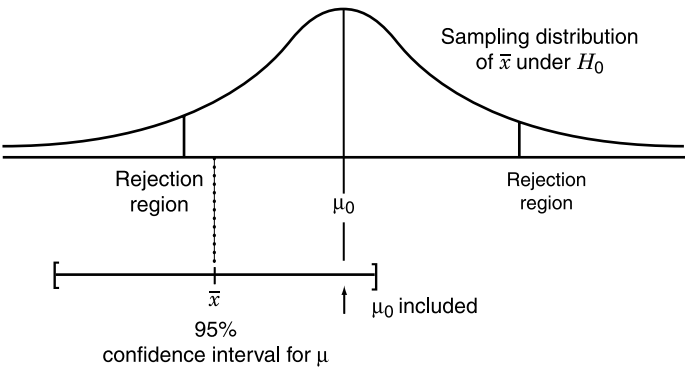
Figure 5.8 \mu_0 included in 95% confidence interval for \mu .
