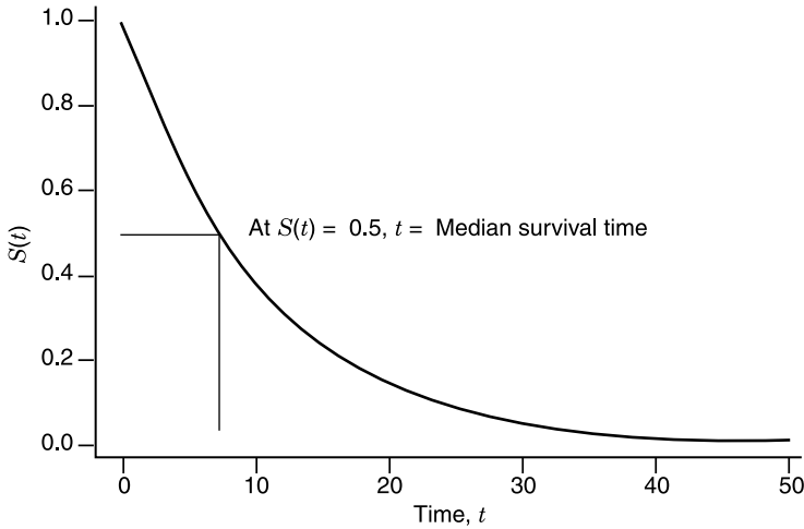
Figure 11.2 General form of a survival curve.
