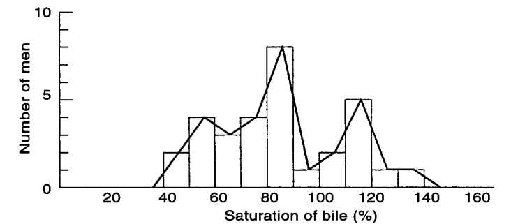
Figure 2.4 Frequency polygon for percentage saturation of bile in men.
