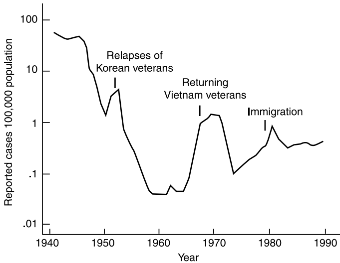
Figure 1.6 Malaria rates in the United States, 1940–1989.
