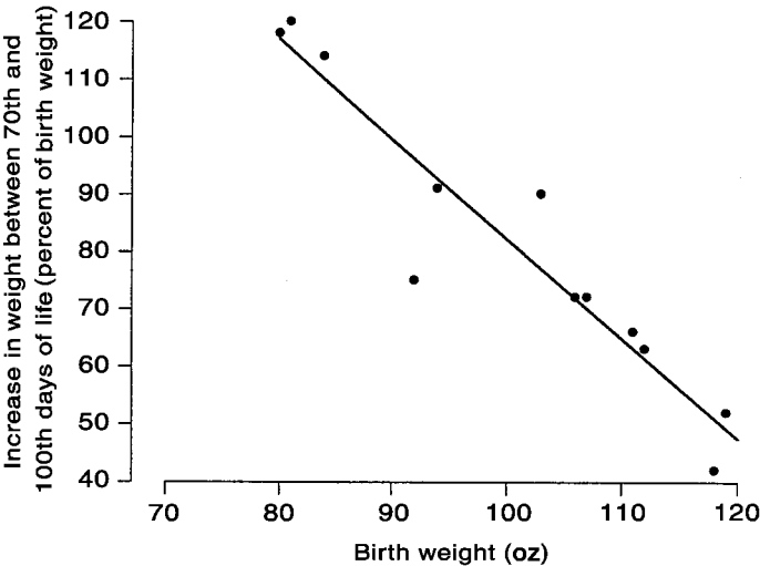
Figure 8.1 Graphical display for data in Example 8.1.
