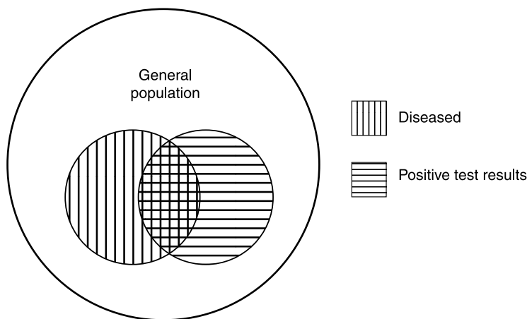
Figure 1.1 Graphical display of a screening test.
