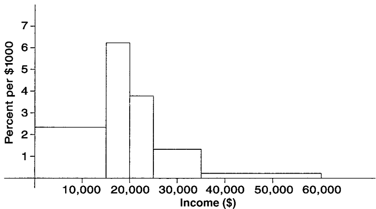
Figure 2.5 Income of U.S. nonwhite families, 1983.
